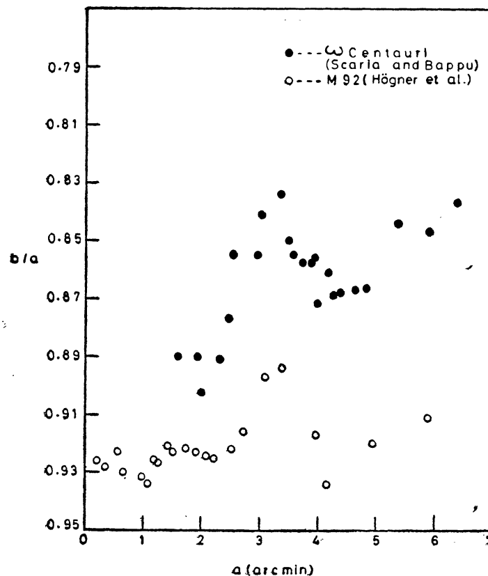
Figure 12. The relationship between b/a and a for the clusters \omega Cen and M 92. Values of semimajor axis a for M 92 have been normalised to the distance of \omega Cen. The data for M 92 is taken from Högner et al. (1973).
