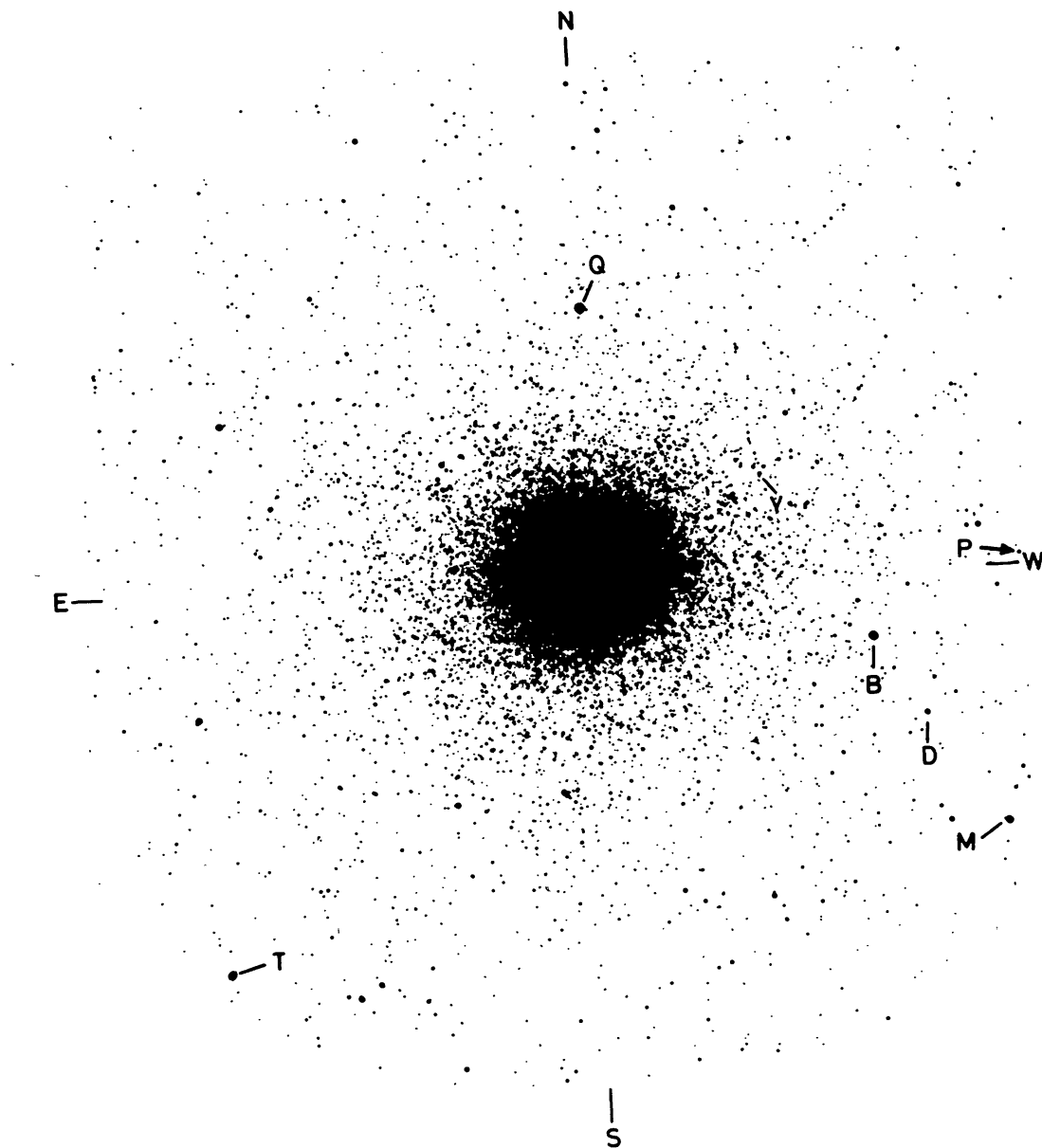
Figure 14. \omega Cen in B Band taken with the 102 cm reflector at Kavalur. Stars marked T and M are the reference stars for the equidensitometry of the cluster. Star P is the reference star for the scan in the east-west direction and star Q is reference star for the north-south scan. Stars B and D are the two photoelectric standards. Star Y has been identified in Fig. 15(b) which shows the distribution of blue stars.
