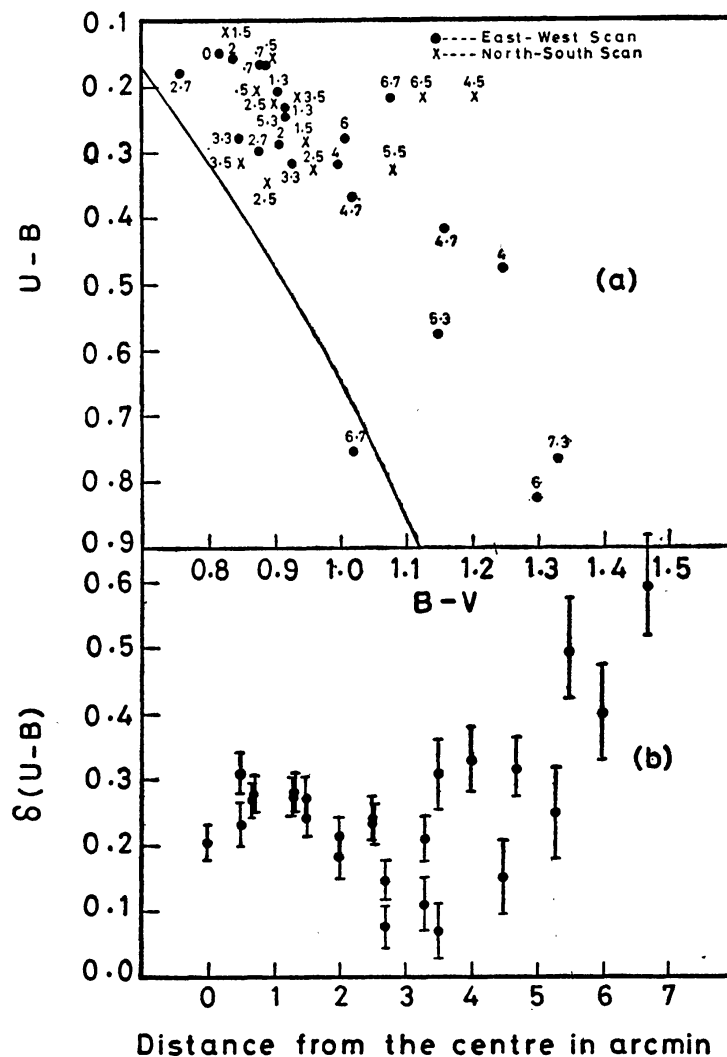
Figure 6. (a) U-B , B-V relation for the observed regions of the cluster \omega Cen. The number marked against each point is the distance in minutes of arc from the centre of the cluster. (b) The dependence of the UV excess of these regions on their distance from the centre. The sampling error in U-B is shown by vertical bars.
