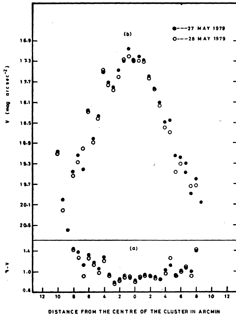
Figure 2. V magnitudes and B - V colours obtained on two consecutive nights by an aperture scan of \omega Cen, in the east-west direction. The stability of the counts proves the accuracy of positioning the aperture over the cluster.
