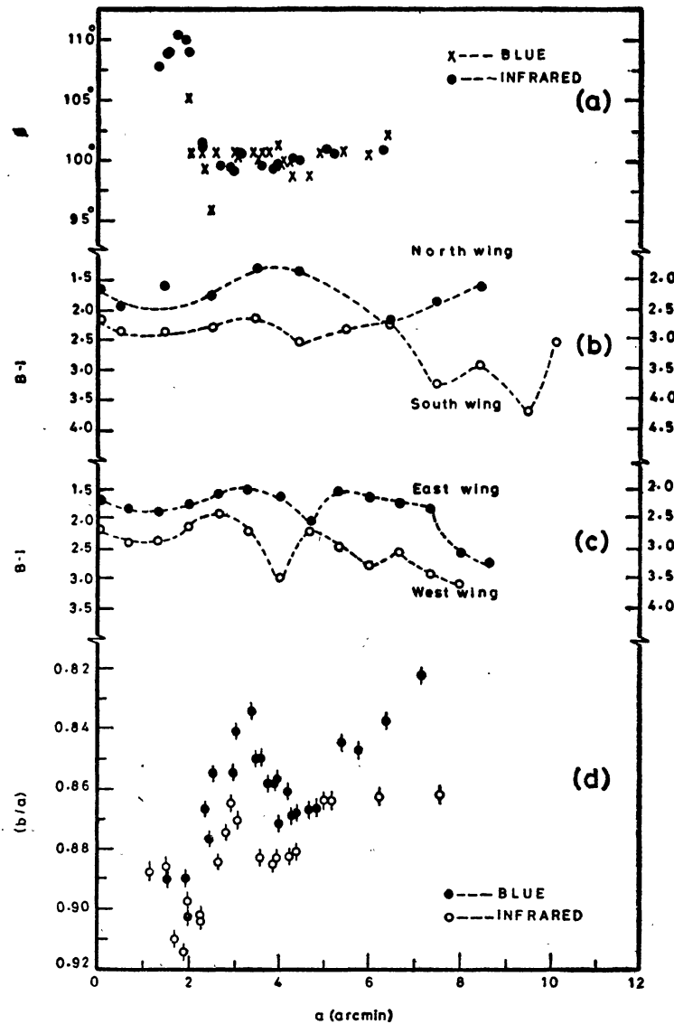
Figure 11. (a) The variation of position angle of the major axis of the equidensity contours of \omega Cen as a function of the semi major axis ( a ). (b) The variation of B-I colour along the minor axis of \omega Cen. The north wing (scale at right) and the south wing (scale at left) are separately shown. (c) The variation of B-I colour along the major axis of \omega Cen. The east wing (scale at right) and the west wing (scale at left) are separately shown. (d) The variation of the axial ratio ( b/a ) of the equidensity contours of \omega Cen as a function of the semimajor axis ( a ).
