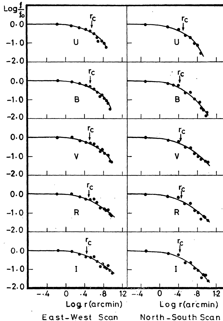
Figure 4. Surface brightness profiles in U , B , V , R and I bands, of \omega Cen, along the major and minor axes. Continuous lines in each figure show the best fitting model of King (1966a). Core radii r_c are marked.
