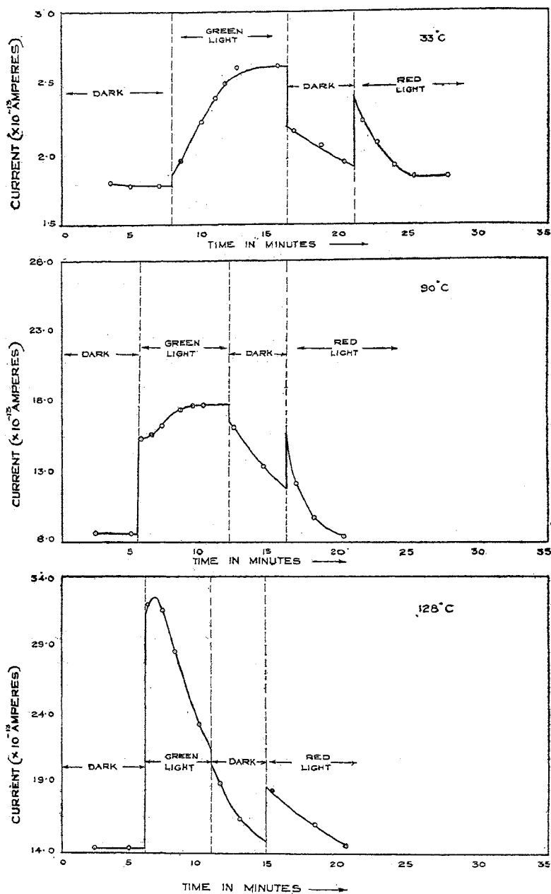
FIG. 5 Variation of photocurrent with temperature
